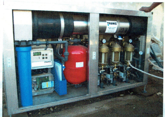
Trunz Water Box – Treatment of contaminated water to clean water, free from virus and bacteria.
